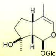
Kankanoside A
