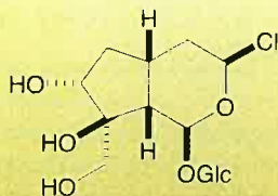
Kankanoside C
