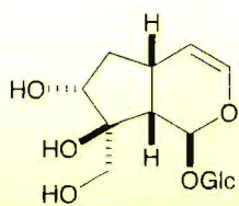
Kankanoside B
