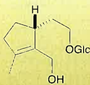
Kankanoside D
