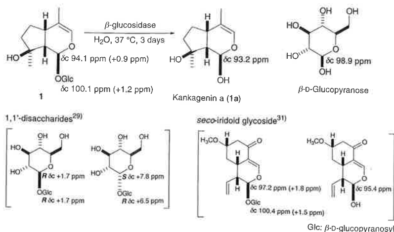
Fig. 3. Application of ^{13}\text{C} -NMR Glycosylation Shift (All in Pyridine- d_5 )
